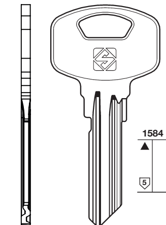
Shoulder milling view
